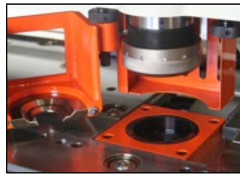
Interchangeable Die-Blocks.
