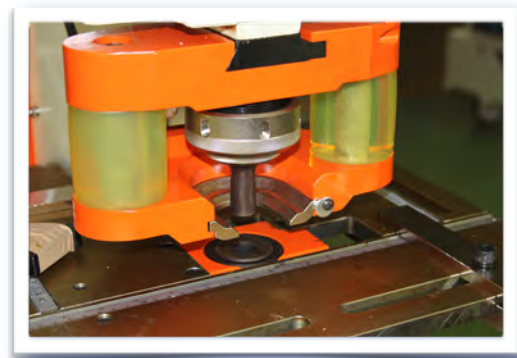
Urethane Stripper
